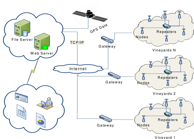
Fig 1: A schematic diagram of WSN layout for modeling the influence of climate change in weather, atmospheric and environmental conditions and on grapevine varieties and wine quality in different styles. The WSN transmits real time data collected through remote, wireless telemetry devices via repeaters, gateways and the Internet to a central sever for display and comparative analysis on the variability in climate change across the world's major wine regions and grapevine varieties.
